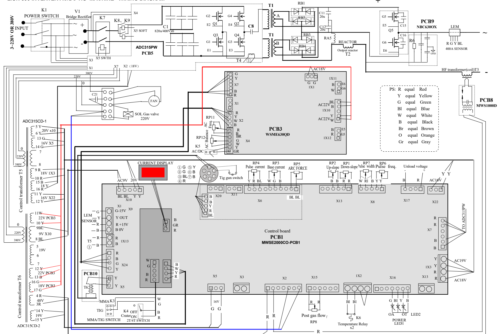
LION 300 INVERTER AC/DC TIG MACHINE WIRING DIAGRAM
